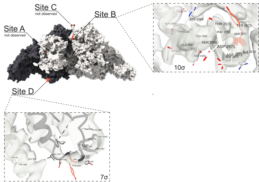
Fig. 6 Location of hormonogenic sites in hTG structure. (Top left) hTG surface representation with one monomer in charcoal and one monomer in white. Acceptor tyrosine residues, Y2573 and Y1310 in ~15 Å proximity 18 at each canonical site (A to D) are marked in red, for which at Y2573, additionally MIT and DIT were detected in MS experiments. The insets show sites B and D in detail with the respective cryo-EM density and its corresponding threshold level to aid confidence assessment.
